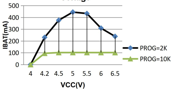
Charge Current VS Supply Voltage
