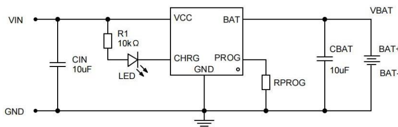
Figure 1. Without absorption circuit
