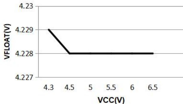
Relationship between float charging voltage and power supply voltage
