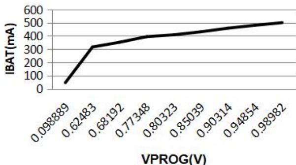
Relationship between charging current and PROG pin voltage
