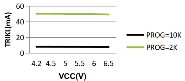
Trickle Charge Current VS Supply Voltage
