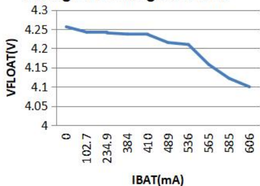
Regulated Output (FLOAT) Voltage VS Charge Current
