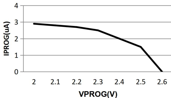
Relationship between PROG pin voltage and PROG pull-up current
