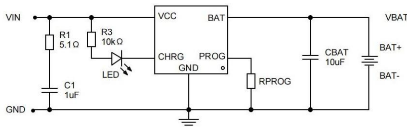
Figure 2. Add absorption circuit
