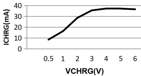
CHRG Pin I-V Curve (Strong Pull-Down State)
