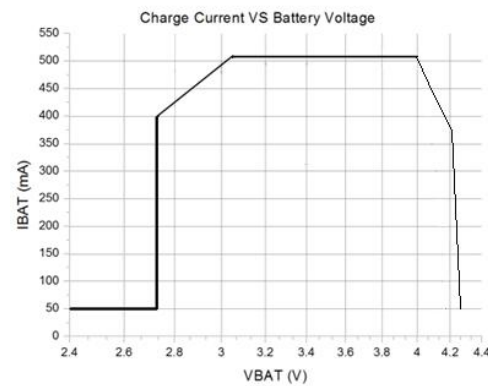
Relationship between charging voltage and charging current
